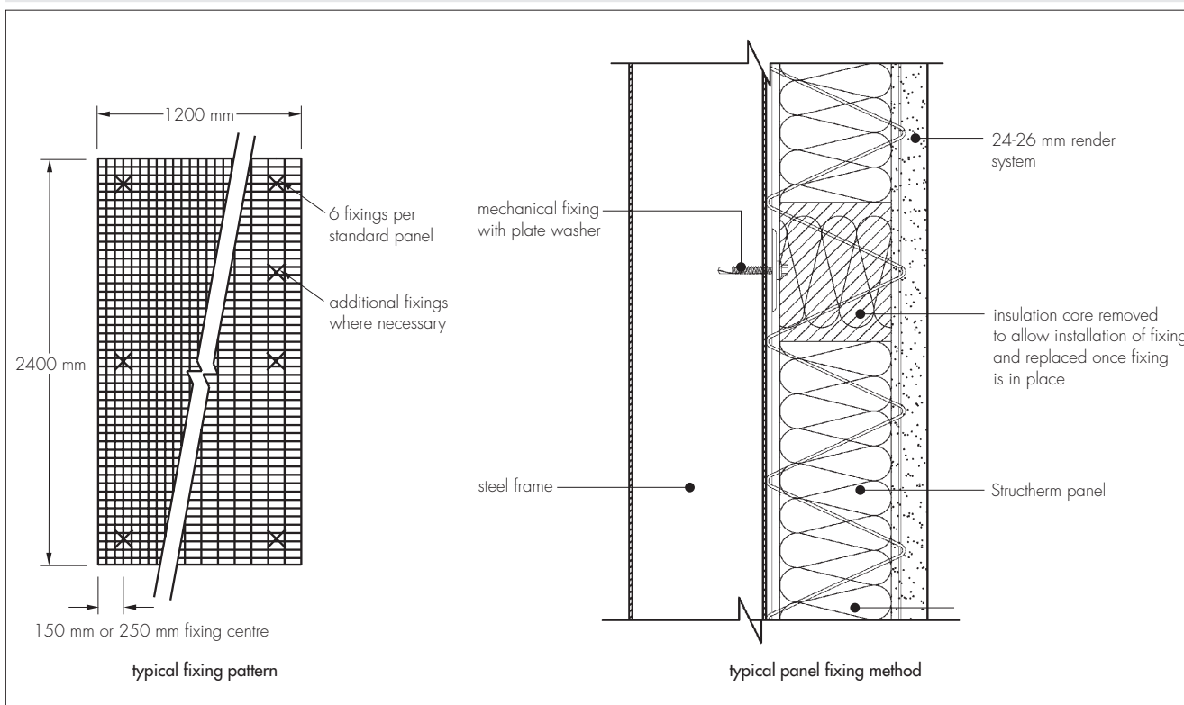
Figure 2 Typical panel fixing pattern
