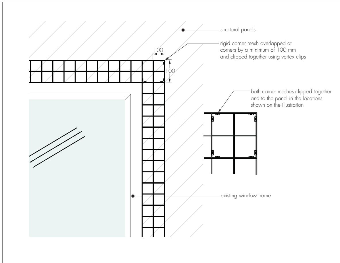
Figure 7 Corner reinforcement
