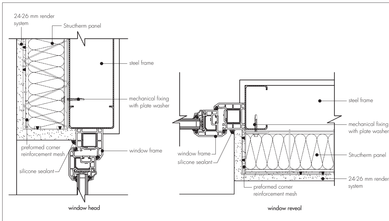
Figure 9 Typical window reveal and head details
