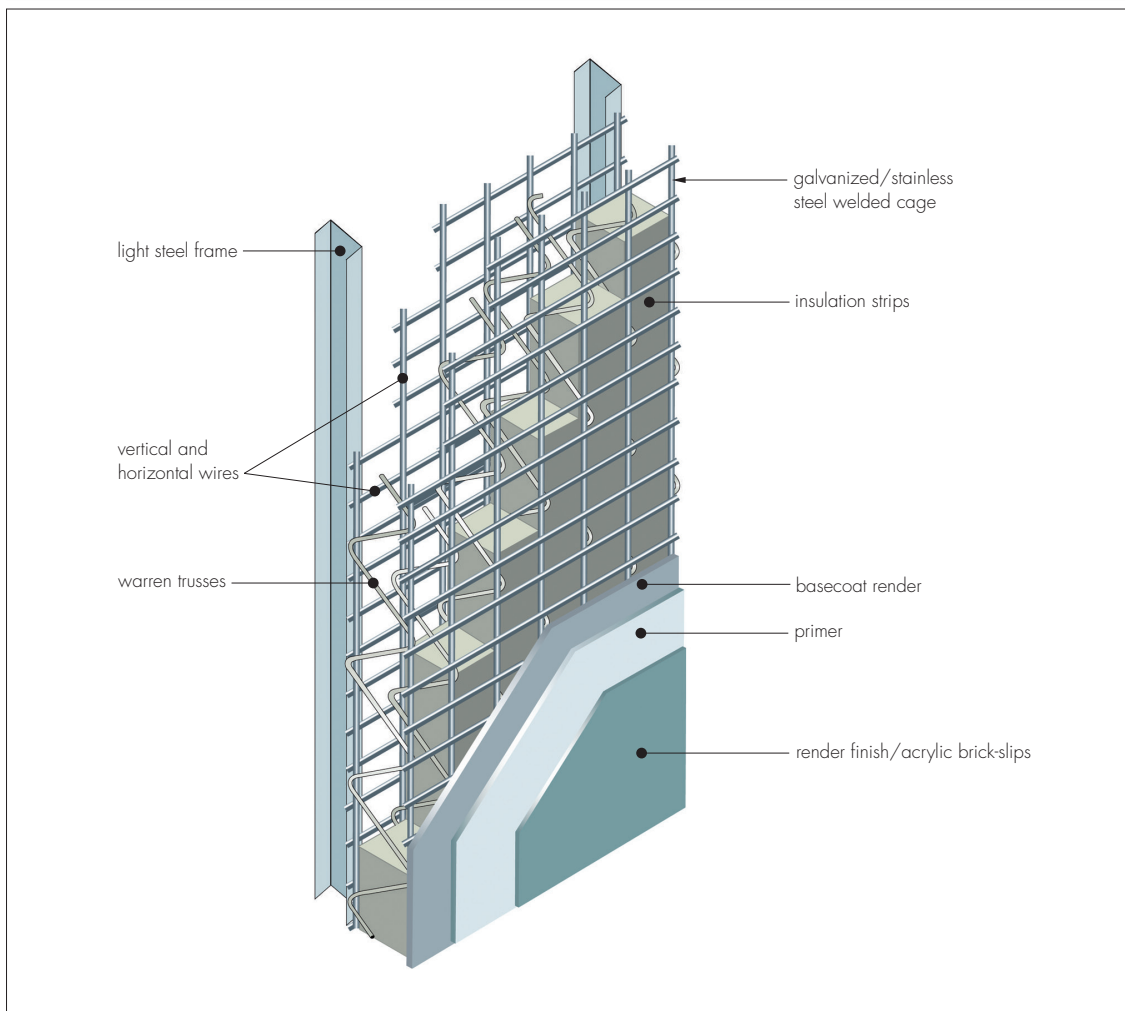
Figure 1 Strutherm Structural Mineral Wool External Wall Insulation System
