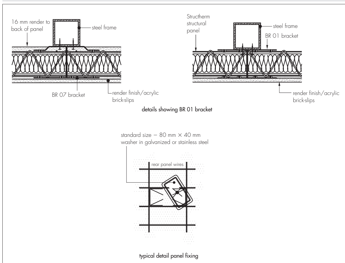
Figure 3 Typical fixing detail
