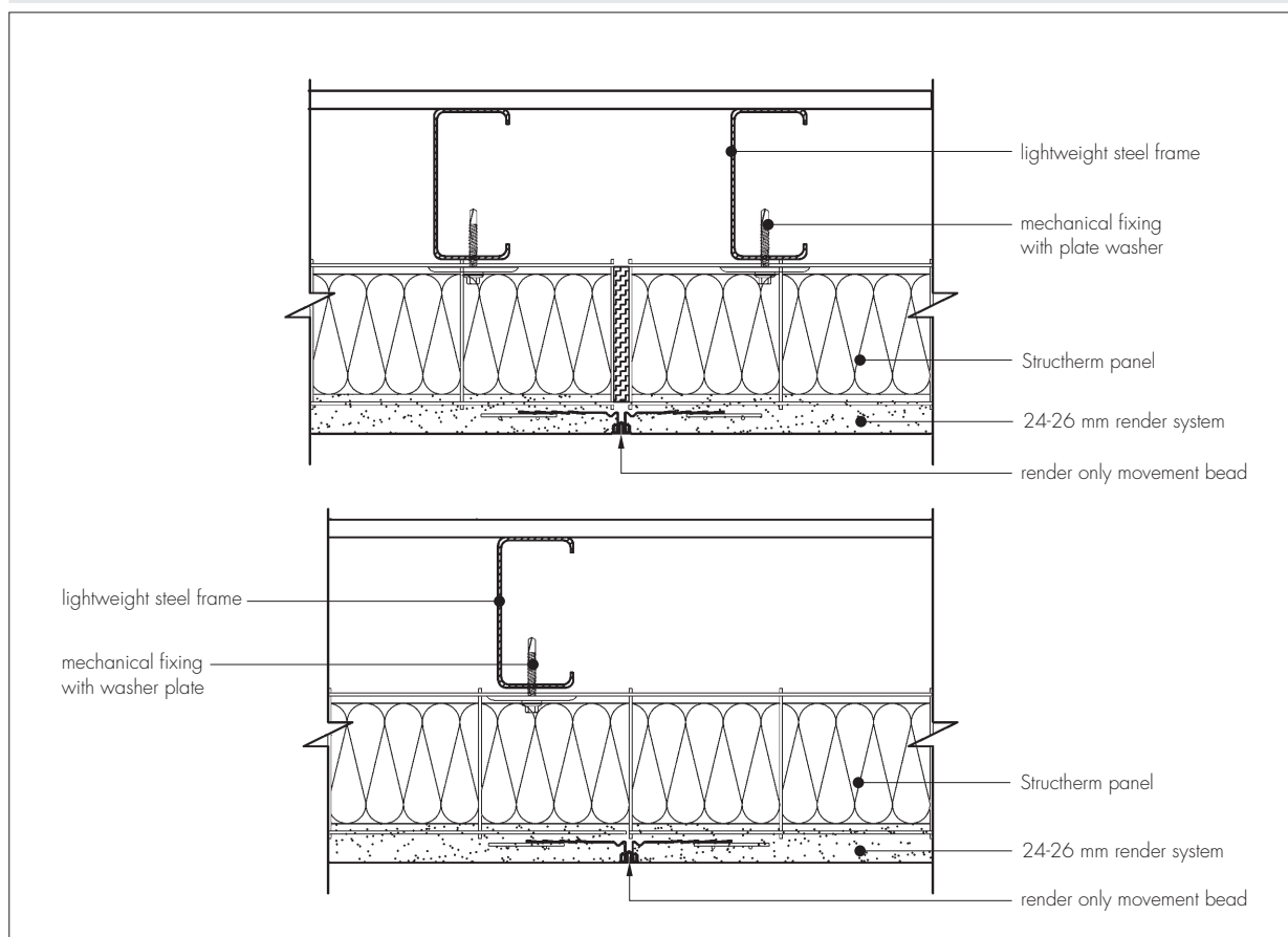
Figure 6 Typical movement joint
