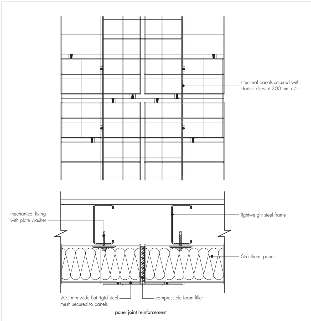
Figure 4 Panel joint reinforcement
