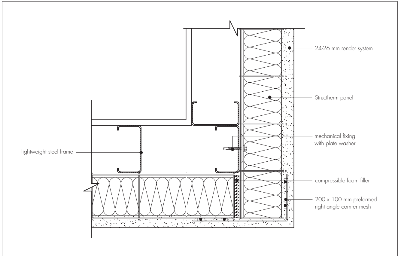
Figure 5 Corner detail
