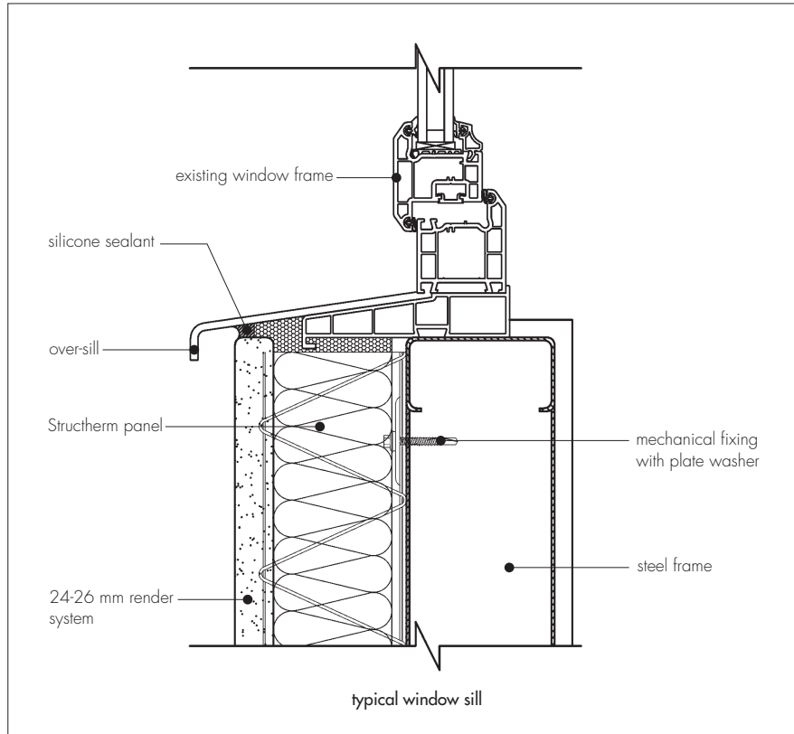
Figure 8 Typical window sill
