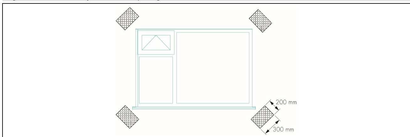
Figure 6 Additional reinforcement at openings
