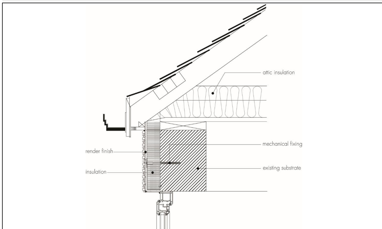
Figure 7 Roof eaves detail
