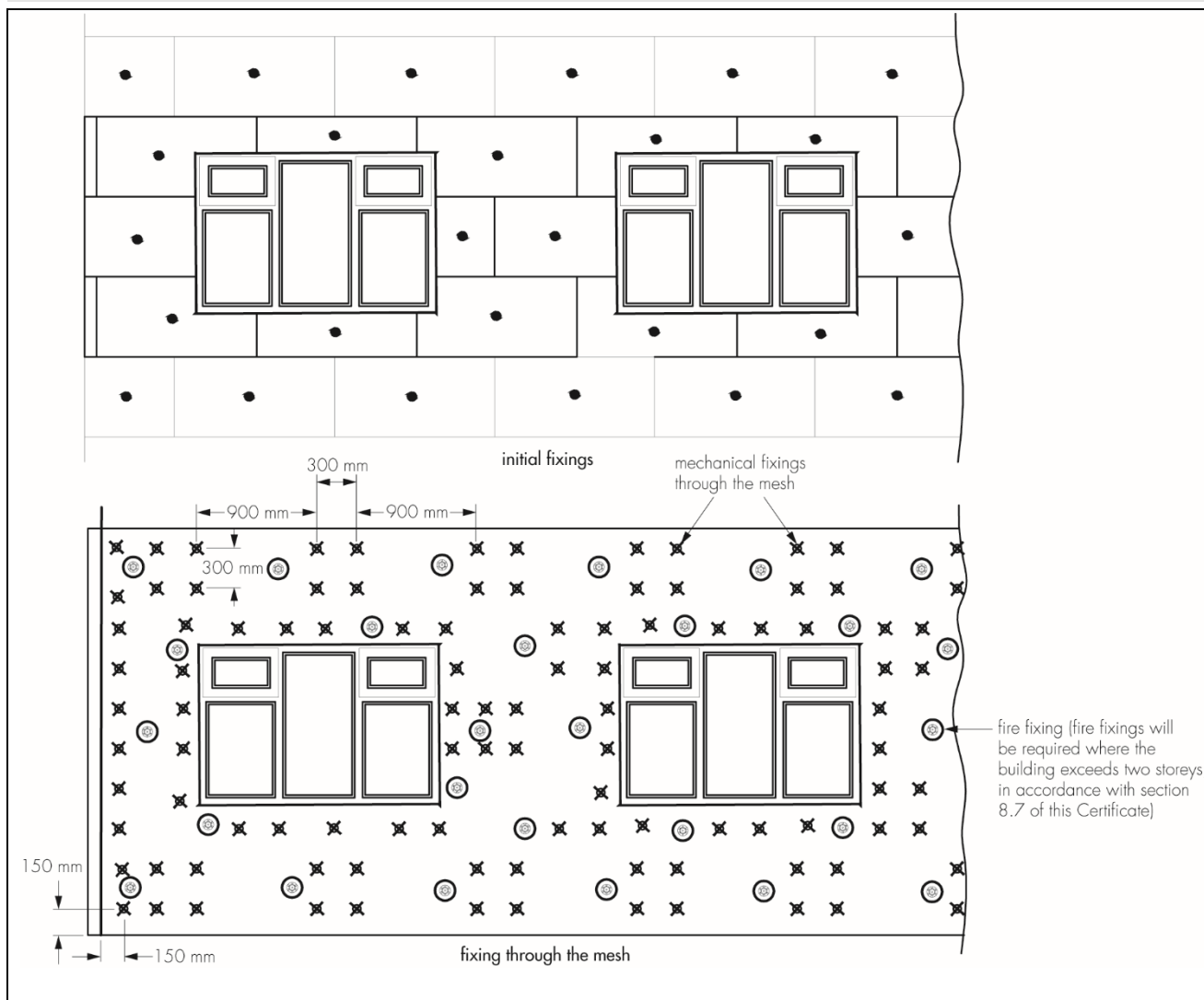
Figure 5 Typical fixing pattern
