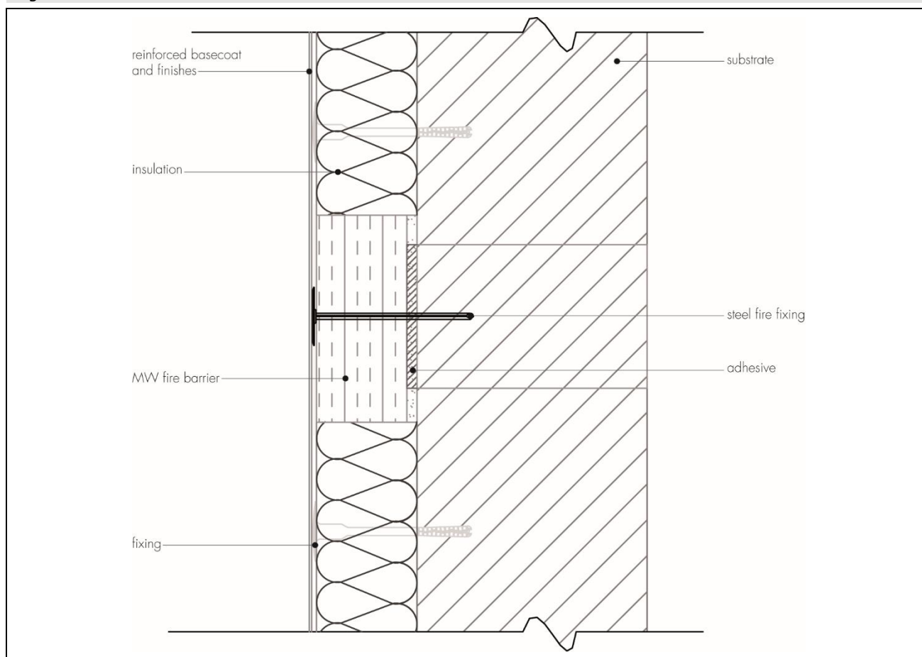
Figure 2 Fire barrier
