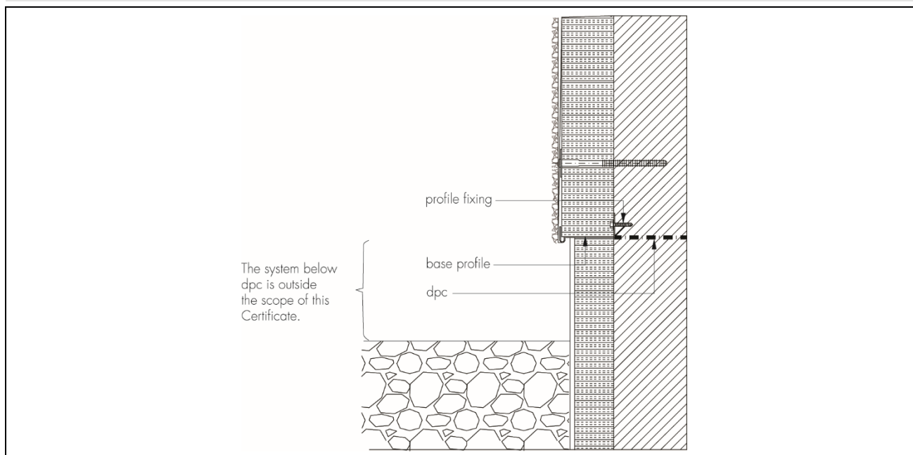
Figure 3 Typical section of base profile
