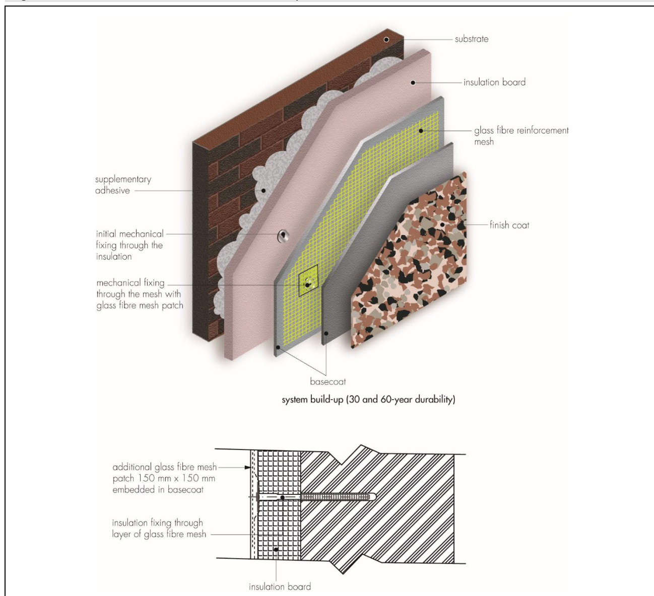
Figure 1 The Struc-Dash P External Wall Insulation System
