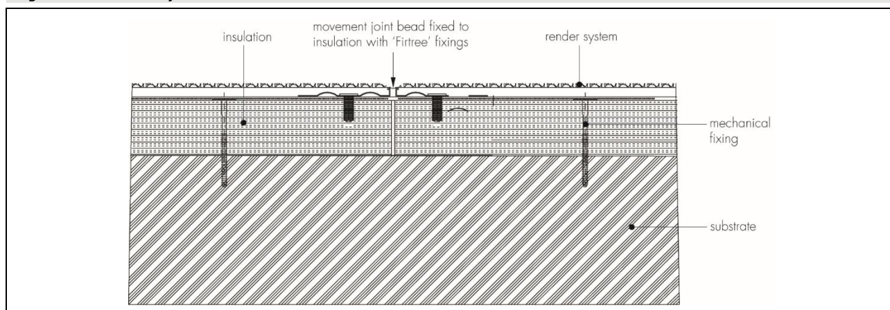
Figure 4 Movement joint detail
