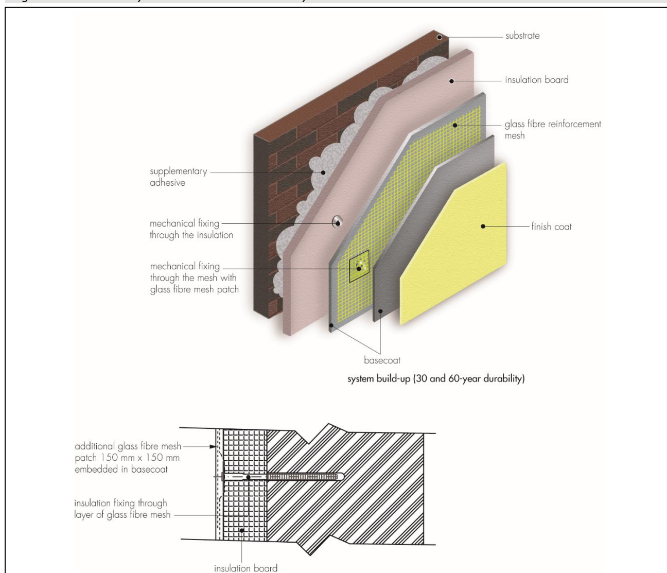
Figure 1 The Struc-Acryl P External Wall Insulation System
