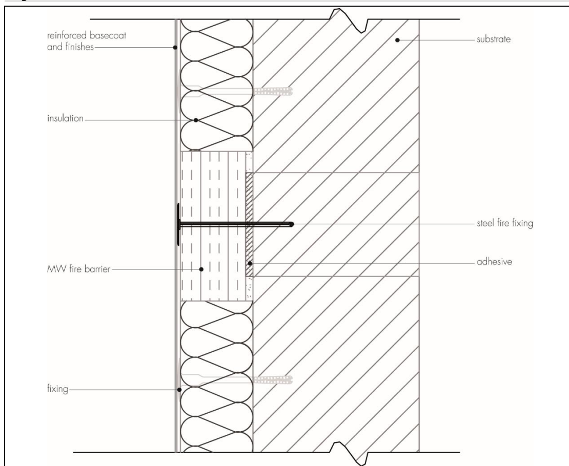
Figure 2 Fire barrier
