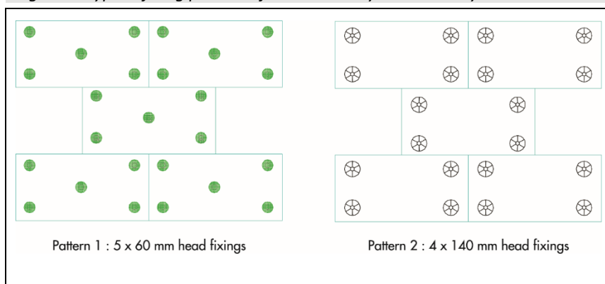
Figure 5 Typical fixing pattern of boards – 30 year durability
