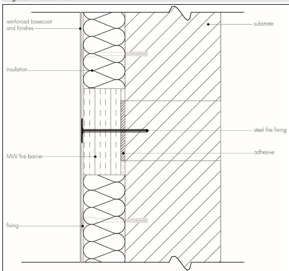
Figure 2 Fire barrier
