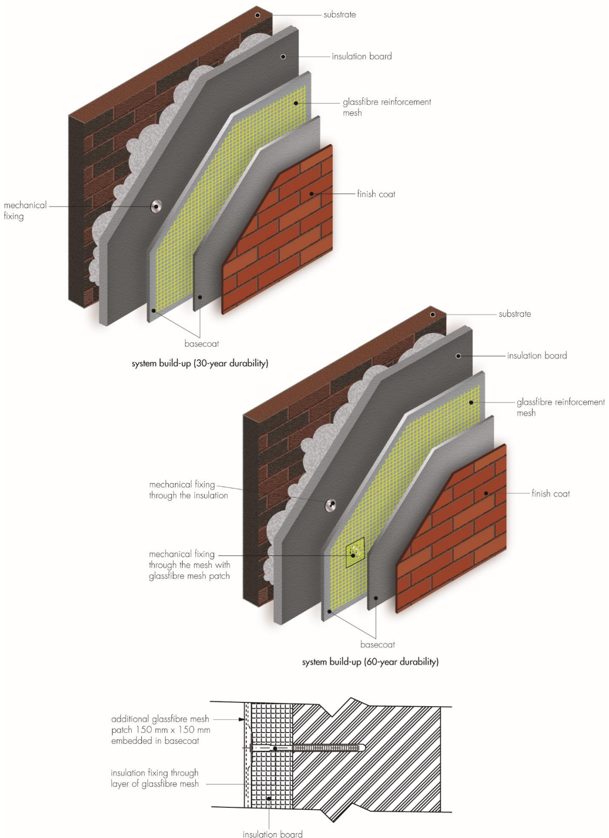
Figure 1 The Struc-Brick Rend E External Wall Insulation System
