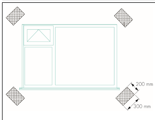
Figure 6 Additional reinforcement at openings
