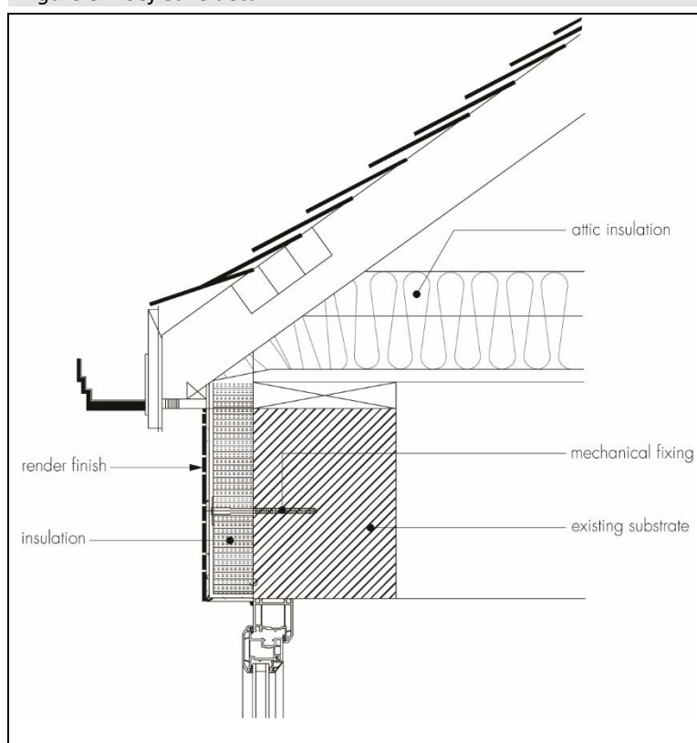
Figure 8 Roof eave detail
