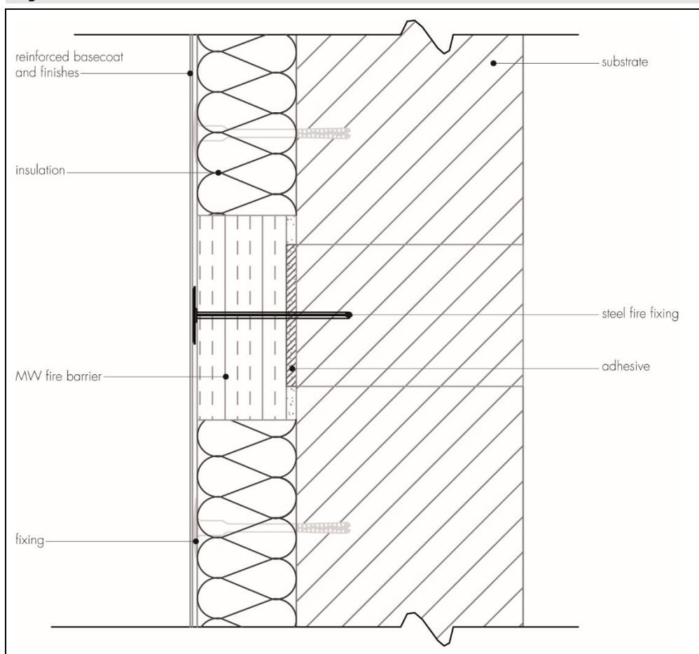
Figure 2 Fire barrier
