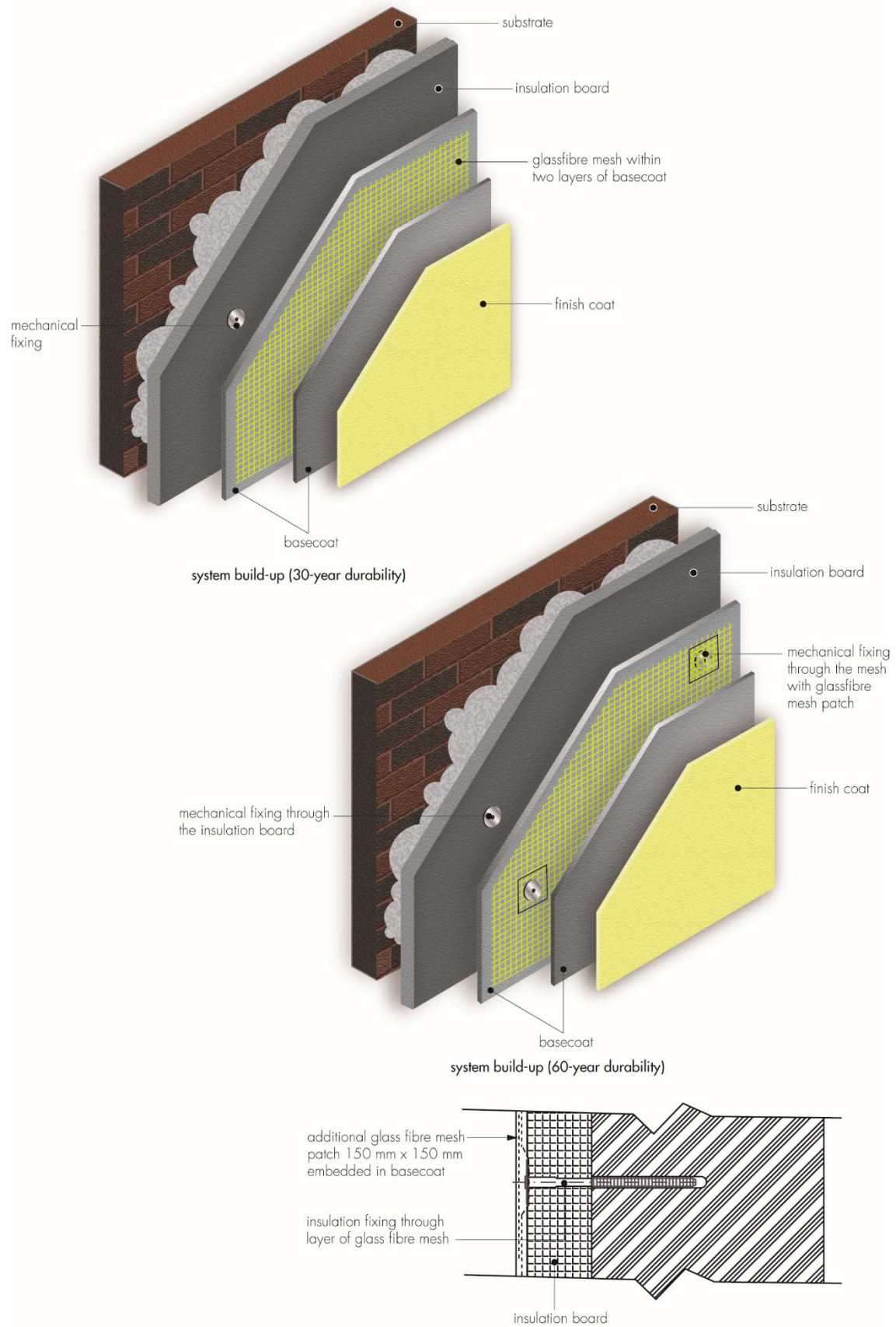
Figure 1 The Struc-Sil E External Wall Insulation System
