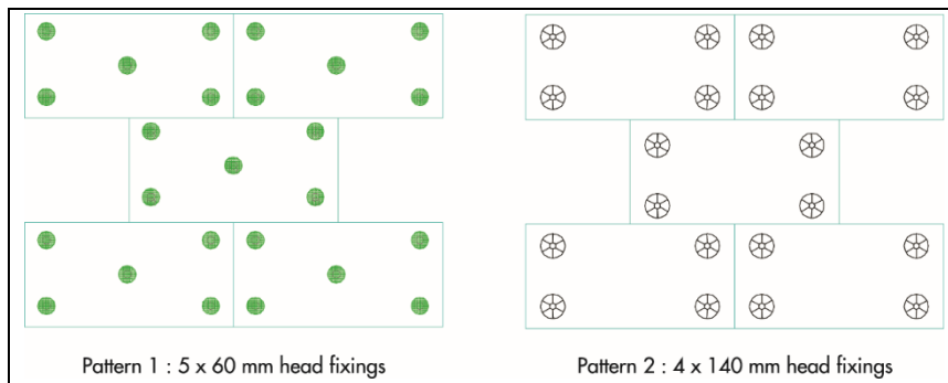
Figure 5 Typical fixing pattern of boards
