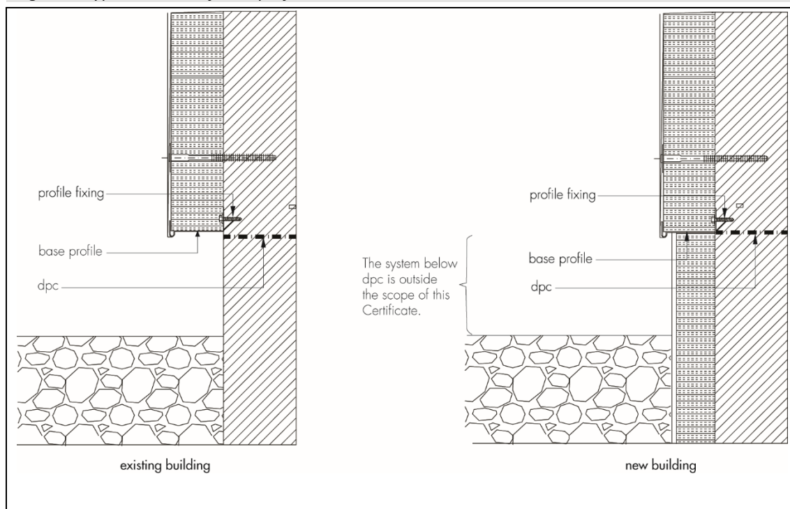
Figure 3 Typical section of base profile
