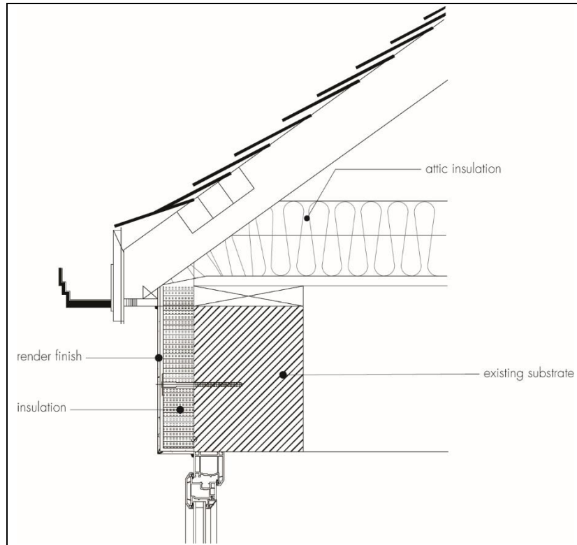
Figure 8 Roof eave detail
