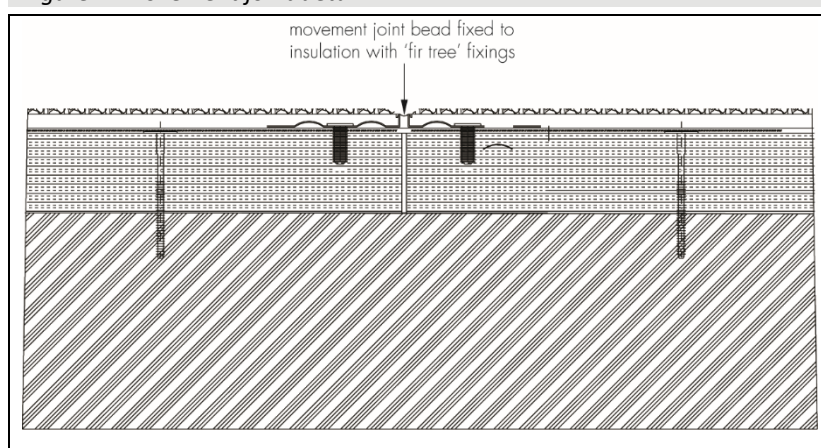
Figure 4 Movement joint detail
