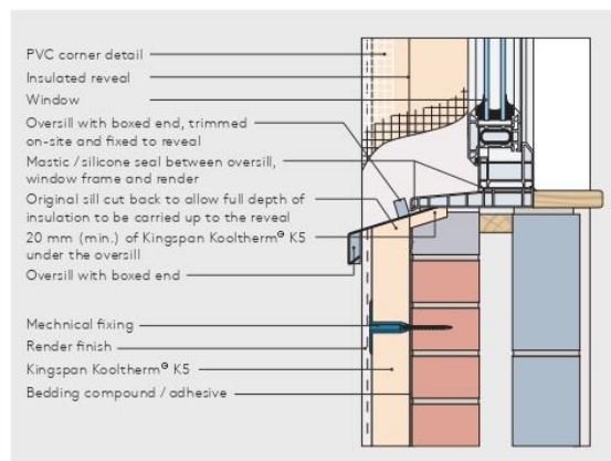
Figure 9 - Overall Extension Detail (Refurbishment)
